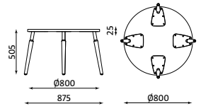
Tauko Coffee Table-LWM Ø 800 weight: 15.20 kg
