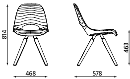
Tauko A-PLUS 4L-LWM weight: 6.20 kg
