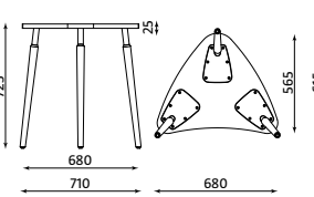
Tauko Modular Table-LWM weight: 9.60 kg
