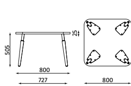
Tauko Coffee Table-LWM 800 x 800 weight: 17.60 kg
