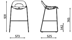
Tauko LB HOCKER CFS-ROD weight: 7.90 kg
