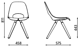
Tauko 4L-LWM weight: 5.60 kg
